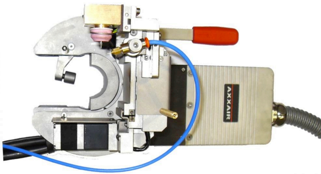
Orbital welding head low package with AVC/OSC
