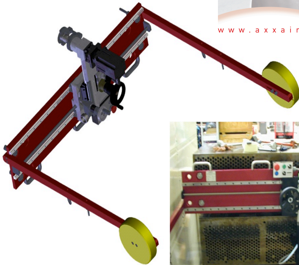
Cutting of inconel tube on Tube Sheet of a heat Exchanger
