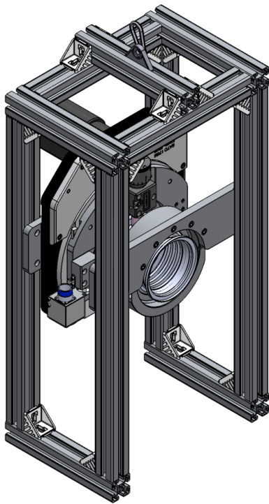
Orbital welding of "SCHOTT" tubes for Solar power station
