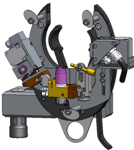
Orbital welding head low package with AVC/OSC
