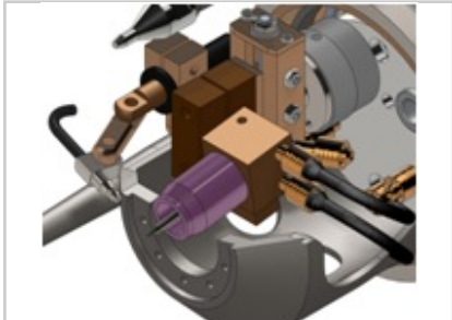
Water-cooled tilt head with adjustable wire
